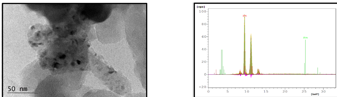
Figure 1. TEM (a) and fluorescence X-Ray (b) analysis of polymer composite with incorporated Pt
