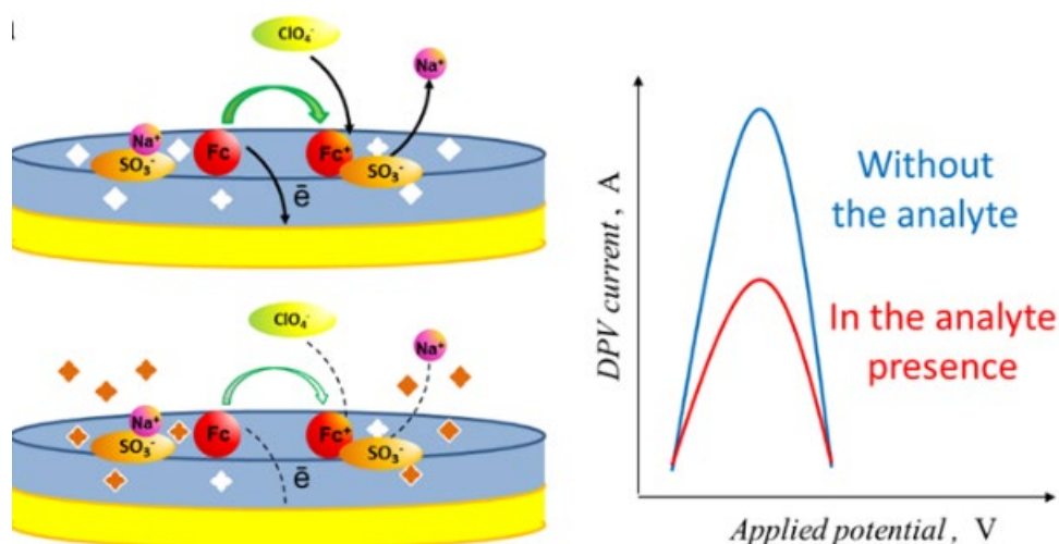
Fig. 1 Application of ferrocene containing MIP in chemosensing.
