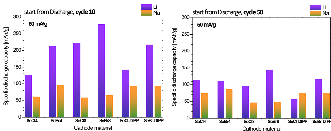
Fig.1 Discharge capacity of NIs cycled in lithium half-cells (blue bars) and sodium half-cells (orange bars) for the 10th and 50th cycle, starting from a discharging mode at current load 50 mA/g.
