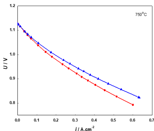
Fig. 1 Current-voltage ( i-v ) curves of the aged cell before 20 redox cycles (▲) and after 20 redox cycles (●).
