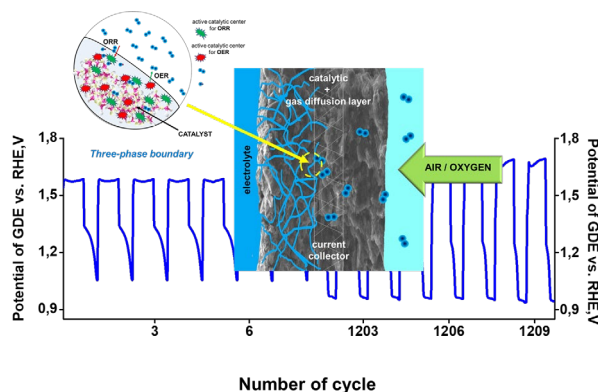
Fig. 1 Schematic figure of the single-layer GDE and cyclic stability test.
