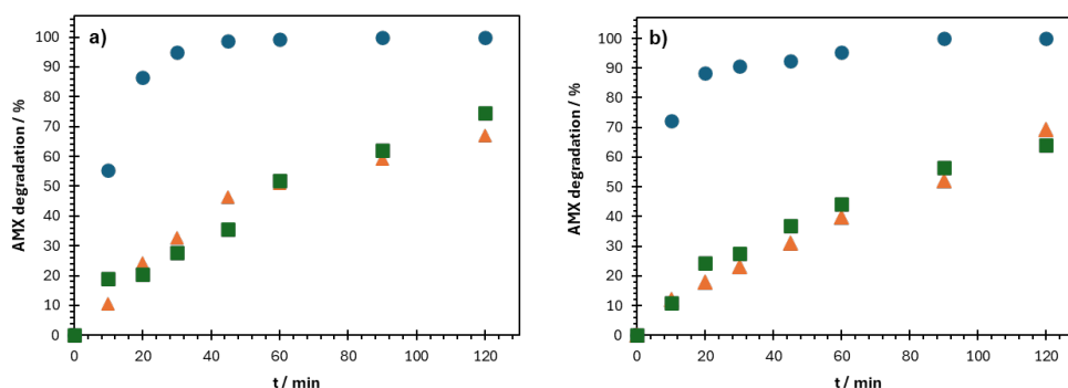
Fig. 1 Influence of tert-butanol and isopropanol as scavengers on the time course of AMX degradation percentage using carbon-based cathodes. Toray ® carbon paper cathode modified with (CEM) from PA (a) and SR (b), without scavenger (●), tert-butanol (▲), and isopropanol (■). Current density: 0.85 mA cm -2 , supporting electrolyte: \text{Na}_2\text{SO}_4 0.1 M, 200 rpm, and 24 °C.
