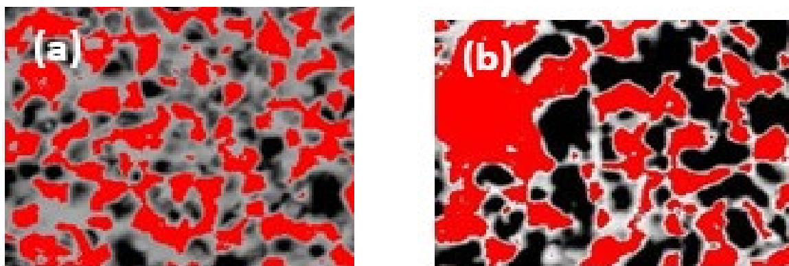
Fig. 3 SEM-BSE images: a) pristine cell b) cell after 20 redox cycles (red – Ni; black – pores; grey – YSZ) ( 2\mu\text{m} resolution).
