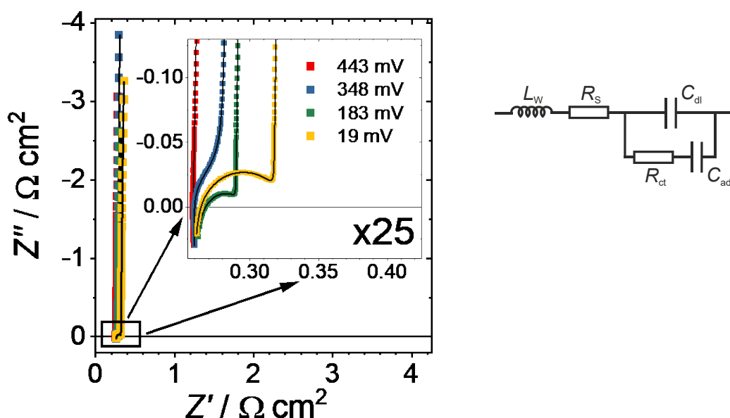
Fig. 1. (left) Complex plane plot of impedance spectra for Pt(111) in 0.5 M H_2SO_4 . Symbols represent experimental data; solid lines are fits of equivalent circuit (right). L_w – inductance of the electrical connections, R_s – solution resistance, C_{dl} – double layer capacitance, R_{ct} and C_{ads} – hydrogen electrosorption charge transfer resistance and capacitance.
