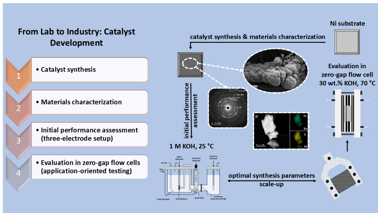
Figure 1 Schematic representation of catalyst development from laboratory-scale to industrial application.
