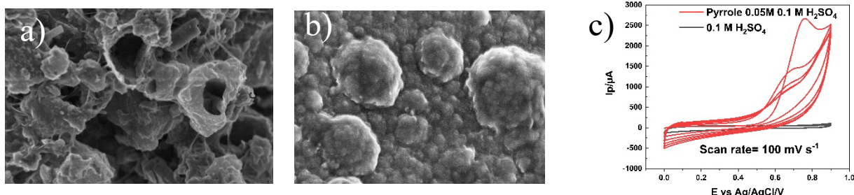
Fig. 1 a) SEM micrograph of the AC; b) SEM micrograph of the Ppy, c) cyclic voltammograms recorded during the electropolymerization of pyrrole on the modified electrode.
