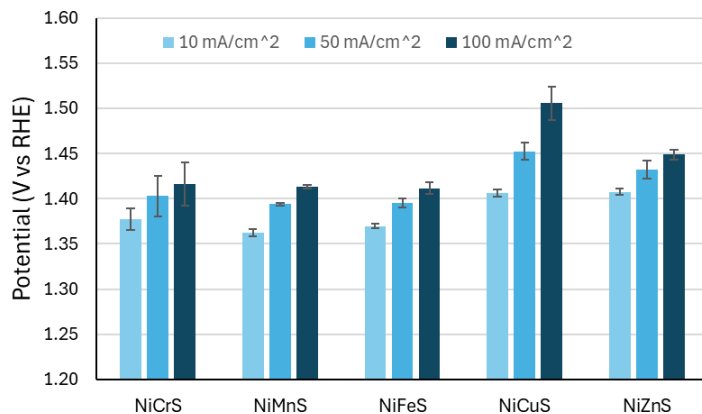
Fig. 1 Required potential at different current densities for transition metal containing Ni sulfide electrocatalysts on Ni foam under alkaline UOR conditions (1 M KOH + 0.33 M urea).
