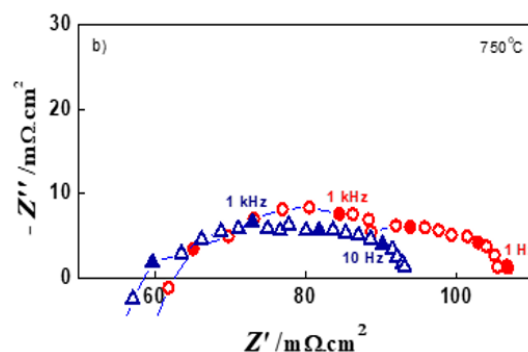
Fig. 2 EIS diagram: before degradation (▲) and after degradation (●) under load of 0.5 \text{ A cm}^{-2} .
