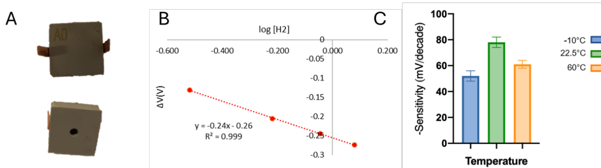
Fig. 1 A) Picture of the solid-state hydrogen sensor. B) Typical calibration curve; the variation of the potential is shown as a function of the concentration of hydrogen. C) Sensitivity of the sensor as a function of the temperature in the range -10 to 60 °C.
