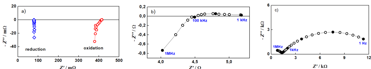
Fig. 4 Oxidized and reduced states of bare anode at 750^{\circ}\text{C} (a), 2 min. oxidation/24 min in \text{N}_2 flow (b), 5 min. oxidation/270 min in \text{N}_2 flow (c).
