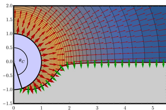
Fig. 1 Carbon corrosion simulation.
