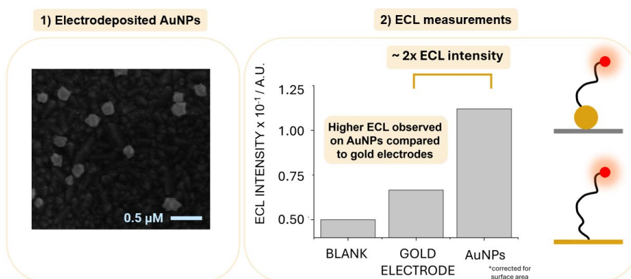
Fig. 1 SEM image of electrodeposited AuNPs. 2) ECL measurement of immobilized \text{Ru}(\text{bpy})_3^{2+} luminophores.
