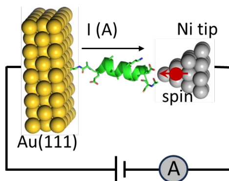
Fig. 1 Schematic illustration of a single-molecule scanning tunnelling microscopy break-junction (STM-BJ) setup, where an \alpha -helical peptide bridges an Au(111) substrate and a magnetic Ni tip for spin-dependent charge transport measurements.
