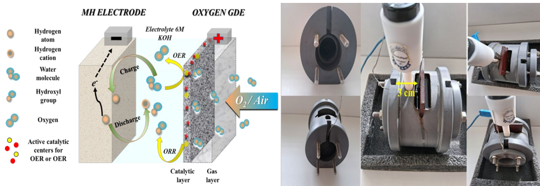
Fig. 1 Schematic representation of the MH-Air battery, the reactions taking place within it, and a photo of its prototype
