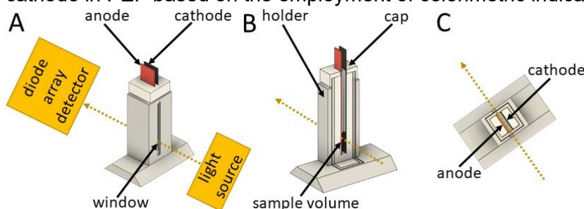
Fig. 1 SEC cell for measurements of pH changes induced by PEF developed and applied in this work. Overall arrangement (A), vertical (B) and (C) horizontal cross-section of the cell.
