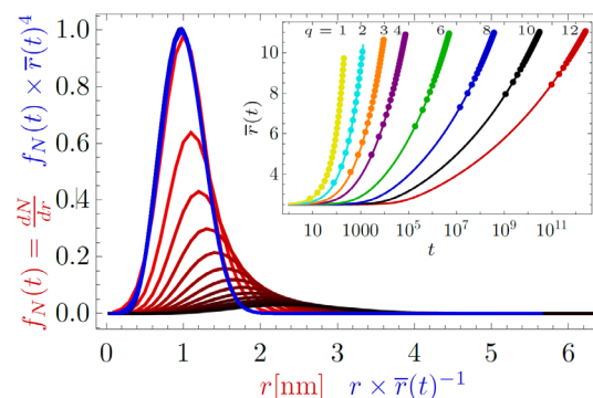
Fig. 2 PSD and mean particle size evolution.
