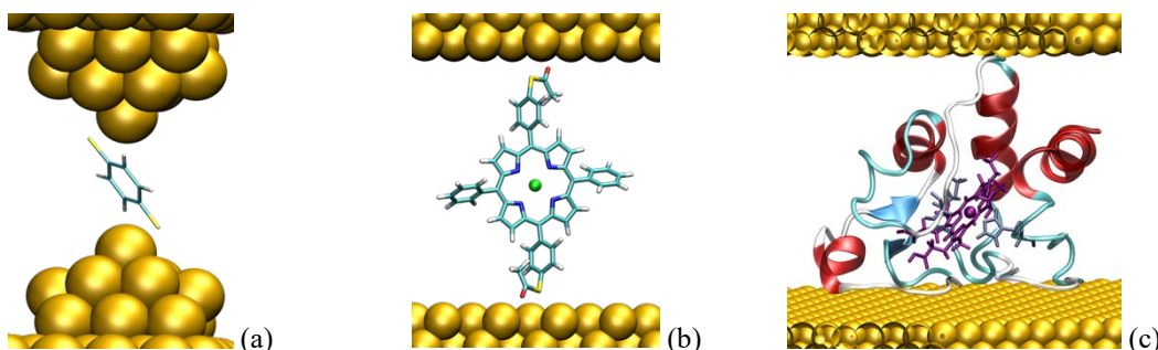
Fig. 1 Atomistic models of (a) benzene-1,4-dithiolate bridge (BDT), (b) Zn-porphyrin junction (ZnTPP), and (c) cytochrome c between two flat gold contacts used for electron transport calculations.
