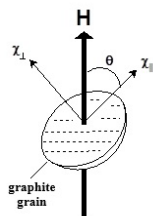
Fig. 1 Diamagnetic ordering of a graphite grain.
