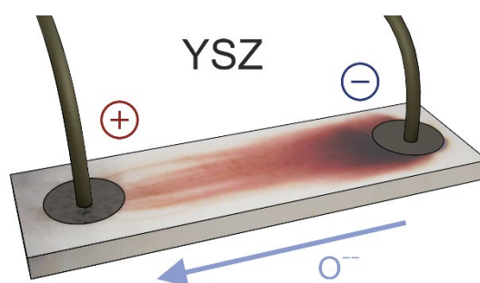
Fig. 1 Illustration of the blackening process in YSZ upon electric polarization.
