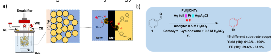
Fig. 1 a) Pickering emulsion system, with CNT-stabilized oil-in-water emulsion on Ag electrode (WE: Working Electrode) enabling interfacial ECHDO of aromatics (where; CE: Counter Electrode, and RE: Reference Electrode). b) Optimized conditions for aldehyde ECHDO across substrates.
