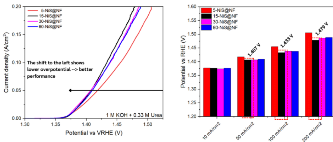
Fig. 1 Required potential at different current densities for NiS@NF electrocatalysts prepared with different number of chemical bath deposition cycles. Conditions: 1 M KOH + 0.33 M urea.
