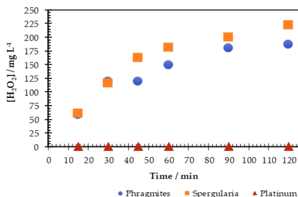
Fig. 2 H 2 O 2 generation over 120 minutes for the functionalized cathodes (CEM) of Phragmites (●) and Spergularia (■) with j = 5.08 \text{ mA cm}^{-2} .
