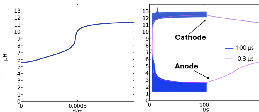
Fig. 1 Spatial distribution of pH across the electrochemical cell at the end of the experiment (i.e., 5 s pre-pulsing, 100 s pulsing, and 100 s post-pulsing period). (Right) Time evolution of pH at the anode and cathode surfaces during water electrolysis in a buffered solution ( \text{pK}_a = 6.94 ).
